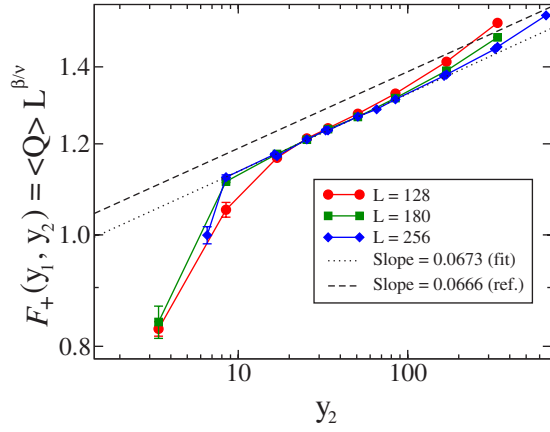
FIG. 4. (Color online) Log-log plot of the scaling function \mathcal{F}_+(y_1, y_2) = \langle Q \rangle L^{\beta\nu} vs y_2 = (H_b/J)L^{\beta\delta\nu} for lattice sizes L=128, 180, and 256 , at the critical period P_c , where y_1=0 . In the L=256 data, near the values y_1=16, 32, 165, and 335 , two closely spaced data points are actually plotted. The best-fit line to the L=256 data in the range 8.46 < y_2 < 84.6 , shown as a dotted line in the plot, corresponds to a scaling exponent 1/\delta_d = 0.0673 \pm 0.0008 . A reference line corresponding to scaling exponent 1/\delta_c = 1/15 = 0.0666 is also shown. These results are in complete agreement with those shown in Fig. 1.
