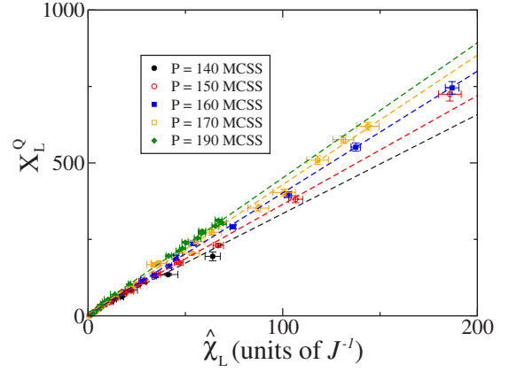
FIG. 5. (Color online) The scaled fluctuations X_L^Q of the dynamic order parameter plotted vs its susceptibility \hat{\chi}_L to the bias field H_b , calculated at L=180 , for periods P=140, 150, 160, 170, and 190 MCSS. The quantity \hat{\chi}_L was calculated using the numerical derivative in Eq. (17). The best-fit lines shown, whose slopes increase monotonically with the period P of the data to which they were fit, were calculated as (3.239J)\hat{\chi}_L + 10.42 , (3.557J)\hat{\chi}_L + 8.735 , (3.980J)\hat{\chi}_L + 3.889 , (4.232J)\hat{\chi}_L + 5.868 , and (4.497J)\hat{\chi}_L + 5.371 , respectively.
