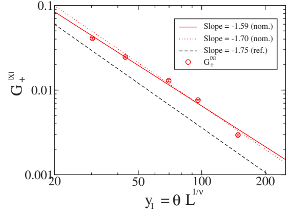
FIG. 11. (Color online) Log-log plot of \mathcal{G}_+^{|X|}(y_1, y_2) vs y_1 , over the range y_1=30.3-149 , for y_2=0 at lattice size L=180 . The relatively small error bars on each data point can be seen inside the larger symbols. The solid and dotted lines are the results of attempts to fit all five and the last four data points with a power-law relationship, and correspond to nominal scaling exponents of -1.59 \pm 0.02 and -1.70 \pm 0.03 , respectively. The dashed line is a reference line corresponding to a scaling exponent of -1.75 .
