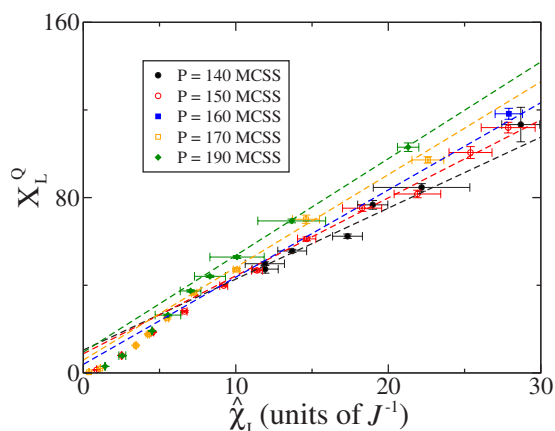
FIG. 6. (Color online) Closeup of Fig. 5, showing the relationship of X_L^Q and \hat{\chi}_L at low values of \hat{\chi}_L , which correspond to large values of the bias field H_b . For P=150, 170, and 190 MCSS, data have been taken (and are shown) down to very low values of \hat{\chi}_L , where the breakdown of the linear relationship between X_L^Q and \hat{\chi}_L can be clearly seen. The dashed lines are the same best-fit lines shown in Fig. 5.
