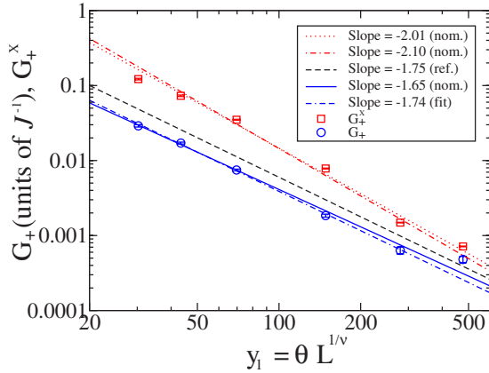
FIG. 10. (Color online) Log-log plots of \mathcal{G}_+(y_1, y_2) and \mathcal{G}_+^X(y_1, y_2) vs y_1 , over the range y_1=30.3-477 , for y_2=0 at lattice size L=180 . The relatively small error bars on each data point can be seen inside the larger symbols. The solid and dash-dash-dotted lines show the result of attempts to fit all six and the first five \mathcal{G}_+ data points, and correspond to a nominal scaling exponent -1.65 \pm 0.03 and a statistically significant scaling exponent -1.74 \pm 0.03 , respectively. The dotted and dash-dotted lines are the result of attempts to fit all six and the first five \mathcal{G}_+^X data points, and correspond to nominal scaling exponents -2.01 \pm 0.01 and -2.10 \pm 0.01 , respectively. The dashed line is a reference line corresponding to the scaling exponent -1.75 .
