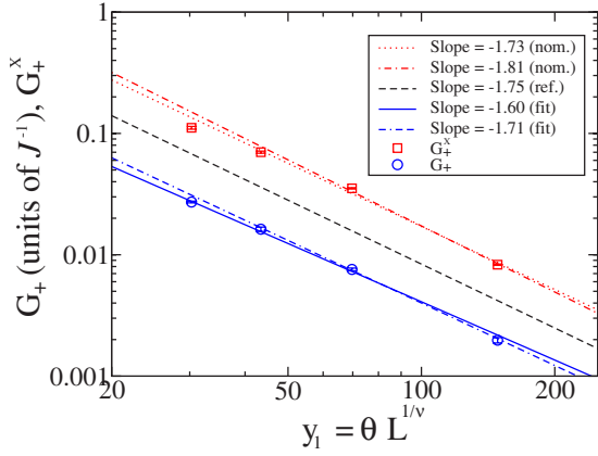
FIG. 9. (Color online) Log-log plots of \mathcal{G}_+(y_1, y_2) and \mathcal{G}_+^X(y_1, y_2) vs y_1 , over the range y_1=30.3-149 , for y_2=8.46 at L=180 . The relatively small error bars on each data point can be seen inside the larger symbols. The solid and dash-dash-dotted lines are fits to all four and the last three \mathcal{G}_+ data points, respectively, and correspond to scaling exponents -1.60 \pm 0.03 and -1.71 \pm 0.05 . The dotted and dash-dotted lines are the result of attempts to fit all four and the last three \mathcal{G}_+^X data points, respectively. They correspond to nominal scaling exponents -1.73 \pm 0.01 and -1.81 \pm 0.02 . The dashed line is a reference line corresponding to scaling exponent -1.75 .
