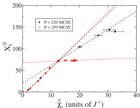
FIG. 7. (Color online) The scaled fluctuations X_L^Q of the dynamic order parameter plotted vs its susceptibility \hat{\chi}_L to the bias field H_b , calculated for lattice size L=180 , at periods P=220 and 250 MCSS. At each period, the data were fit (purely phenomenologically) to two linear relationships. For P=220 MCSS, the fits were calculated as (6.265J)\hat{\chi}_L - 7.497 at low \hat{\chi}_L and (4.161J)\hat{\chi}_L + 19.94 at high \hat{\chi}_L . For P=250 MCSS, the fits were (6.485J)\hat{\chi}_L - 9.240 at low \hat{\chi}_L and (0.2726J)\hat{\chi}_L + 67.92 at high \hat{\chi}_L .
