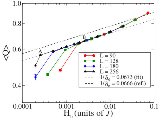
FIG. 1. (Color online) Log-log plot of the dynamic order parameter, \langle Q \rangle , vs bias field, H_b , at P=P_c for L=90, 128, 180 , and 256 . A least-squares fit to power-law scaling of the L=256 data, in the range between the labels A and B above, produced a statistically significant fit with scaling exponent 1/\delta_d=0.0673\pm 0.0008 (corresponding to \delta_d=14.85\pm 0.18 ). The dotted line corresponds to the scaling exponent 1/\delta_d=0.0673 . A reference line representing scaling with the equilibrium Ising exponent, \delta_e=15 ( 1/\delta_e=0.0666 ), is shown as the dashed line.
