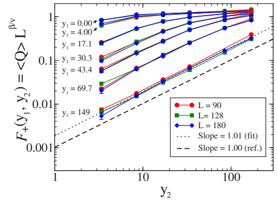
FIG. 3. (Color online) Log-log plot of the scaling function \mathcal{F}_+(y_1, y_2) vs y_2 = (H_b/J)L^{\beta\delta\nu} for lattice sizes L=90, 128, and 180 , for the constant values of y_1 labeled in the plot. The values of y_2 used are y_2=3.39, 8.46, 16.9, 33.9, 84.6, and 169 . The dotted line represents the best fit to the first five points of the L=180 data at y_1=149 and has a slope of 1.01 \pm 0.01 . The dashed line shows the slope value of 1, expected from Eq. (13).
