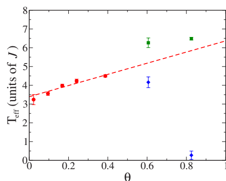
FIG. 8. (Color online) The effective temperature T_{\text{eff}} , obtained as the slopes of the linear fits to the data in Figs. 5 and 7, plotted vs \theta = (P - P_c)/P_c . For the values \theta=0.606 and 0.825 ( P=220 and 250 MCSS), the slopes of both linear regimes fit in Fig. 7 are plotted as T_{\text{eff}} values, using filled squares and diamonds rather than filled circles. The straight line is a weighted least-squares fit to the data below \theta \approx 0.4 ( P < 190 MCSS), and has a slope of 2.97J .
