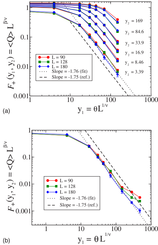
FIG. 2. (Color online) Log-log plots of the scaling function \mathcal{F}_+(y_1, y_2) vs y_1 for lattice sizes L=90, 128, and 180 . The values of y_1 plotted are 4.00, 17.2, 30.3, 43.4, 69.7, 149, and [in (b)] 280 and 477 . (a) The data are shown for the values of y_2 listed on the plot. The best-fit line (dotted) for the last five points of the L=180 data at y_2=3.39 , with slope -1.76 \pm 0.07 , is included along with a reference line (dashed) with the slope -\gamma_e = -1.75 . (b) The data for y_2=3.39 with two additional y_1 values illustrate the boundary of the regime of power-law scaling.
